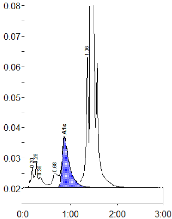
Peak table - ID: 10596757
